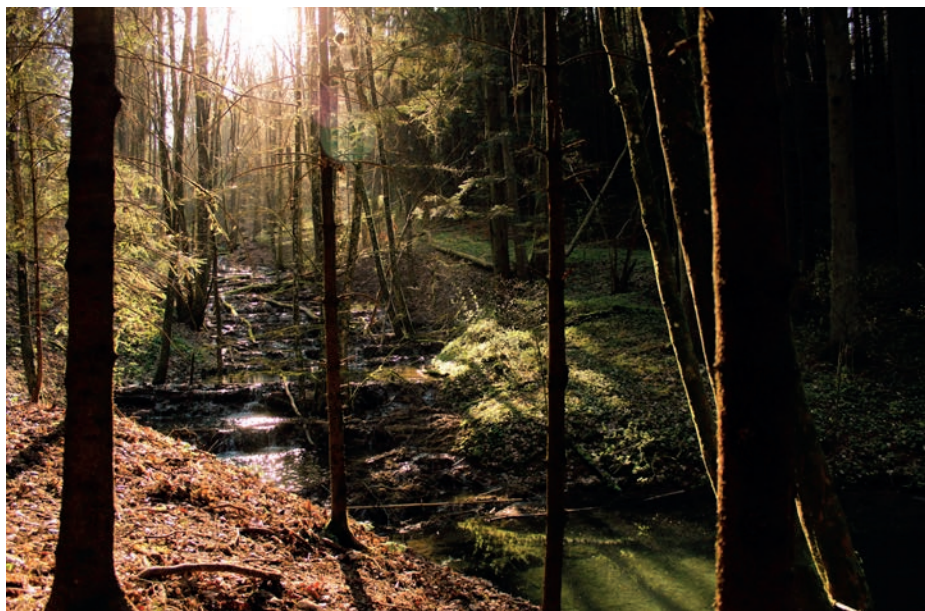
Sinterterrassen in Holnstein
